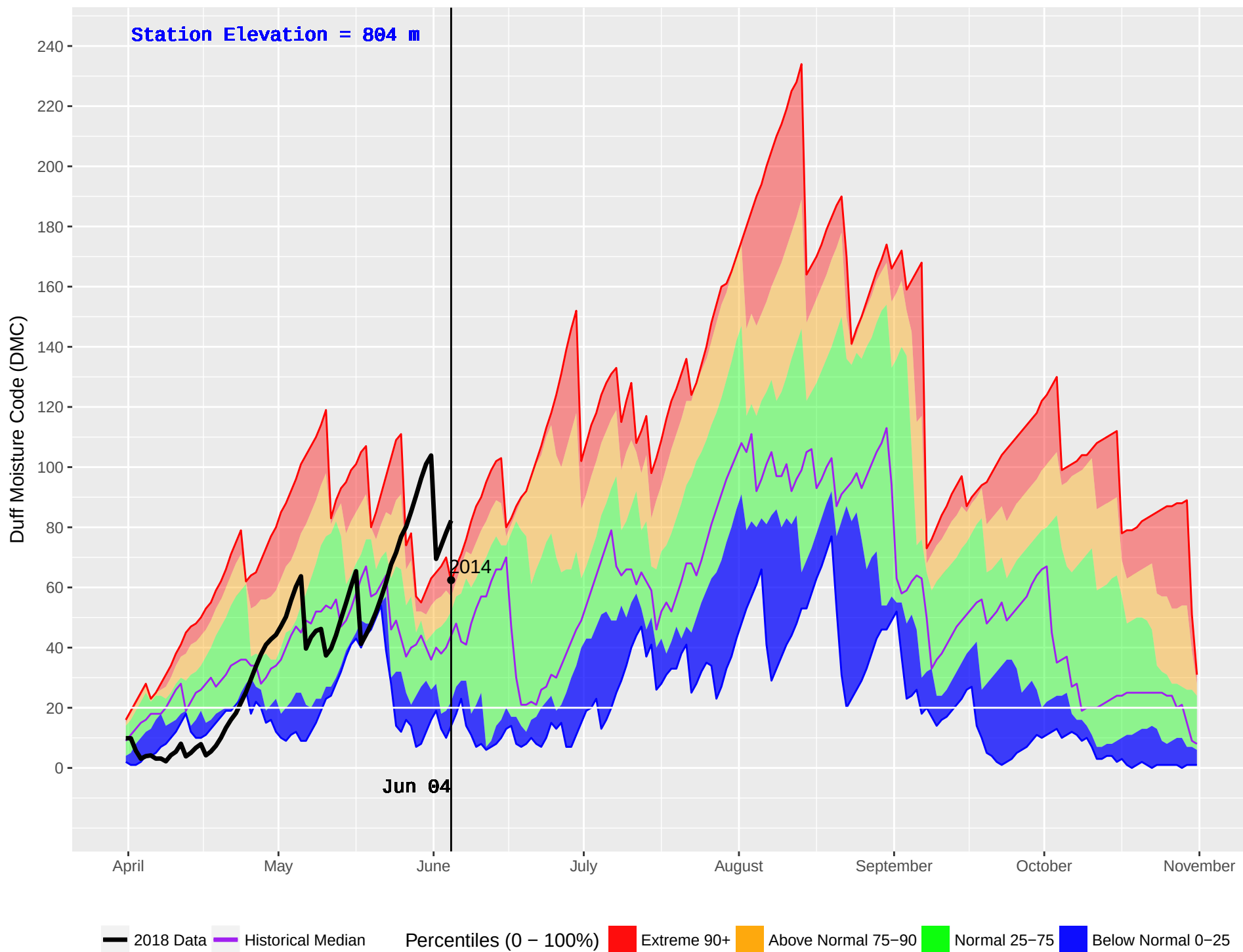
KOOCANUSA (1075) : Historical (2010–2016) and Current (2018) Noon Duff Moisture Code (DMC)
