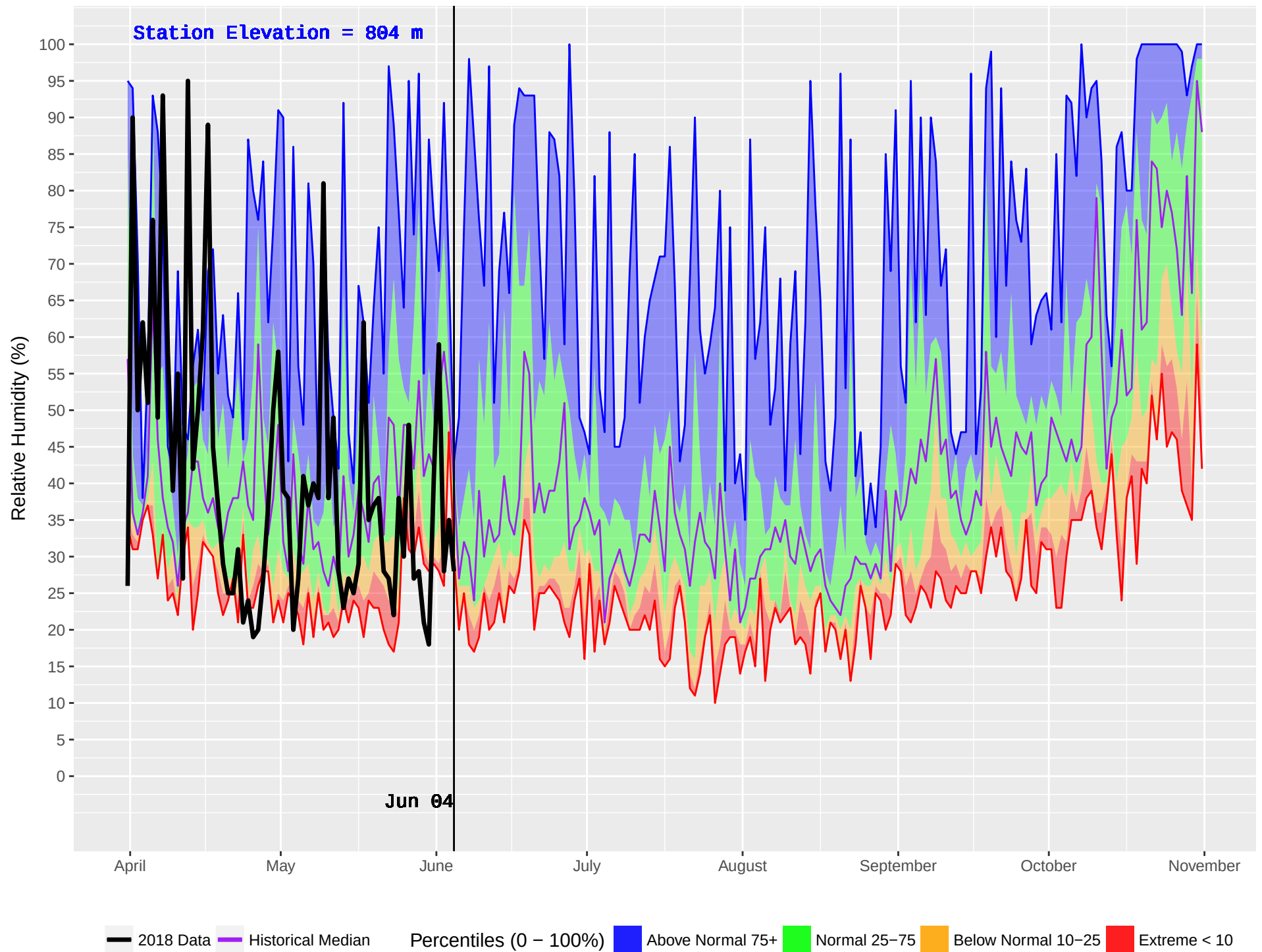
KOOCANUSA (1075) : Historical (2010–2016) and Current (2018) Noon Relative Humidity
